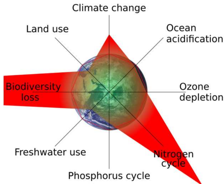
Figure 1. Planetary boundaries according Rockström et al. http://en.wikipedia.org/wiki/Planetary_boundaries . ] The coloured star-like area represents the estimated current state and the corners of the red octagon circumscribed by the Earth are the estimated boundaries. Systems whose safe operating space could not yet be determined were left out.
